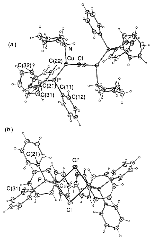
Fig. 1 The molecule of [\{\text{CuCl}(\text{PPh}_3)(\text{pip})\}_2] projected (a) along a line in the \text{CuCl}_2\text{Cu} plane, perpendicular to the \text{Cu}\cdots\text{Cu} line, and (b) normal to this plane. 20% Thermal ellipsoids are shown for the non-hydrogen atoms. Hydrogen atoms have arbitrary radii of 0.1 Å
