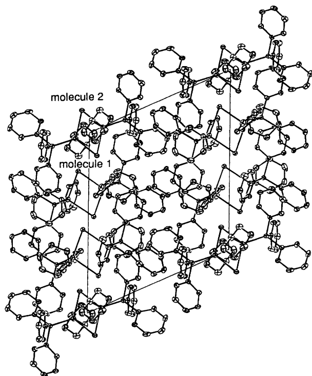
Fig. 2 Unit-cell diagram of [\{\text{CuI}(\text{PPh}_3)(\text{pip})\}_2] projected onto the ac plane
