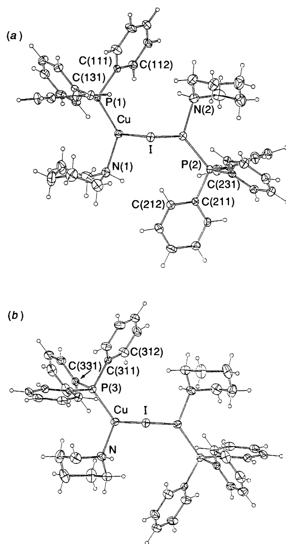
Fig. 3 Structure of (a) the non-centric dimer (molecule 1) and (b) the centric dimer (molecule 2) of [\{\text{CuI}(\text{PPh}_3)(\text{pip})\}_2]
